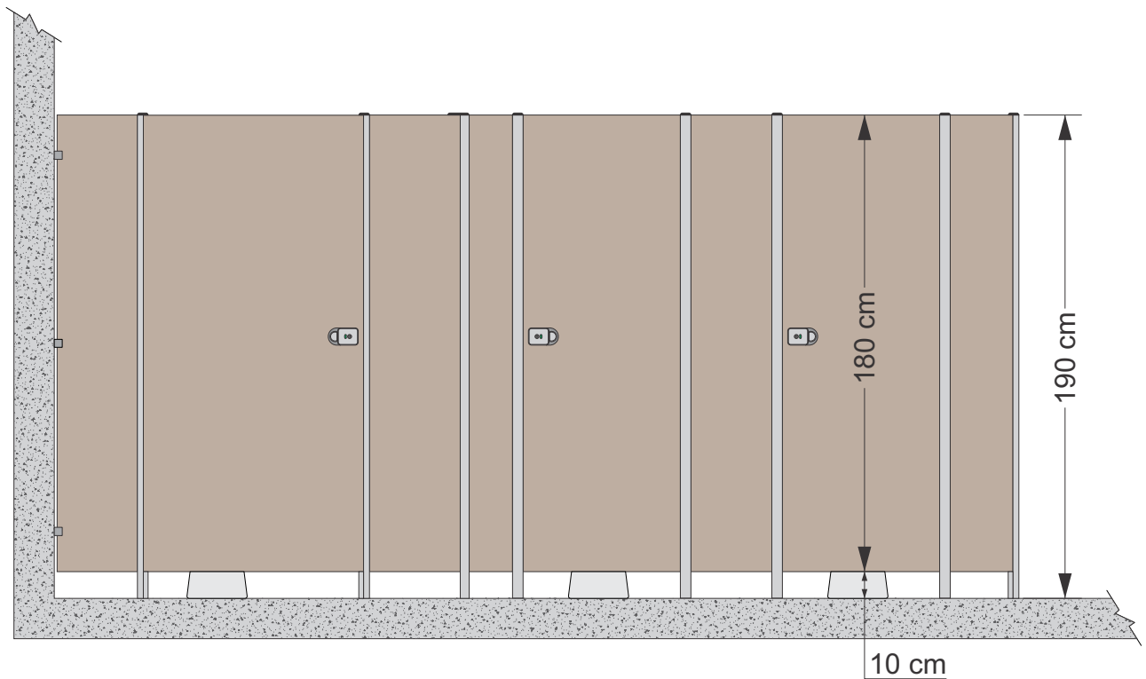
Vista frontal
